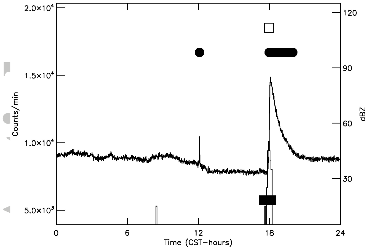
Fig. 1. Summed NaI counting rate per minute in Box 3 on 8/18/2011 (heavy black line, left hand scale). Thin black histogram near the bottom (right hand scale) shows radar reflectivity. The filled rectangle at the bottom marks times of lightning strikes within 5 miles. The row of filled circles near the top marks intervals in which the count rate in 60 sec bins exceeds the day's average by 3 \sigma ; the open square marks the TETRA trigger, i.e., the interval when the rate in 2 msec bins exceeds the day's average by 20 \sigma .
