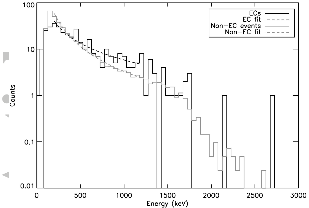
Fig. 5. Spectra of Event Candidates and non-EC TETRA triggers. Spectrum of ECs is shown in black. Spectrum of non-EC TETRA triggers (triggers not associated with lightning nearby in time and distance) is shown in grey. Power law fits between 200 keV and 1200 keV of the form E^{-\alpha} are shown with dotted lines, where \alpha = 1.20 \pm 0.13 and 1.79 \pm 0.04 for EC and non-EC events respectively.
