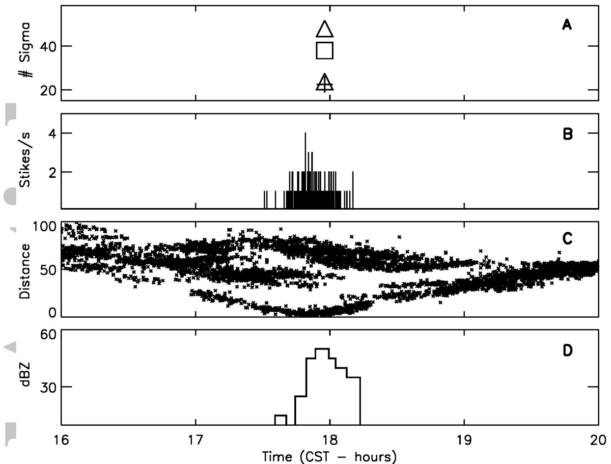
Fig. 3. TETRA Report for 8/18/2011 events. Panel A (top): Triggers detected on 8/18/2011 (NaI signals above 50 keV in a single detector box with count rate per 2 msec in excess of 20\sigma above the 8/18/2011 daily mean counting rate). Box 1 triggers are indicated by plus signs, Box 3 by triangles and Box 4 by squares. Panel B: Rate per second of USPLN lightning strikes within 5 miles. Panel C: Distance to each recorded lightning strike within 100 miles. Panel D: Overhead cloud density.
