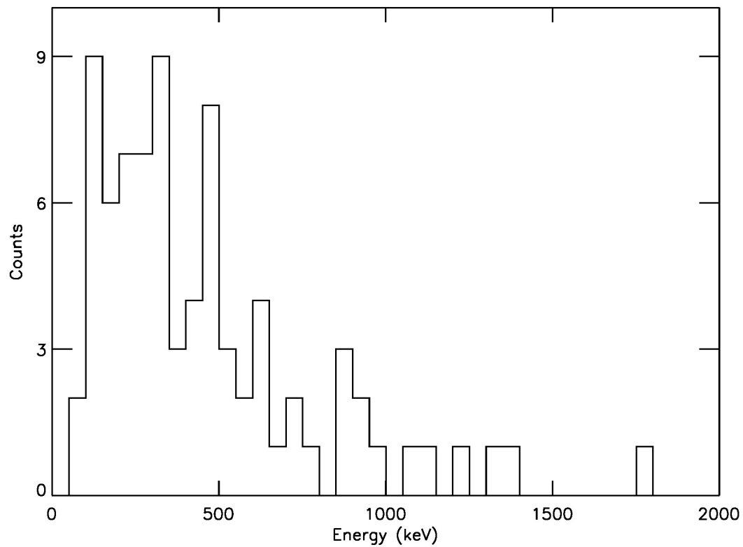
Fig. 7. CEC Event Spectra. Combined NaI detector energy spectrum for the three CECs. 80 photons were detected within the T_{90} interval of each individual detector box's trigger time.
