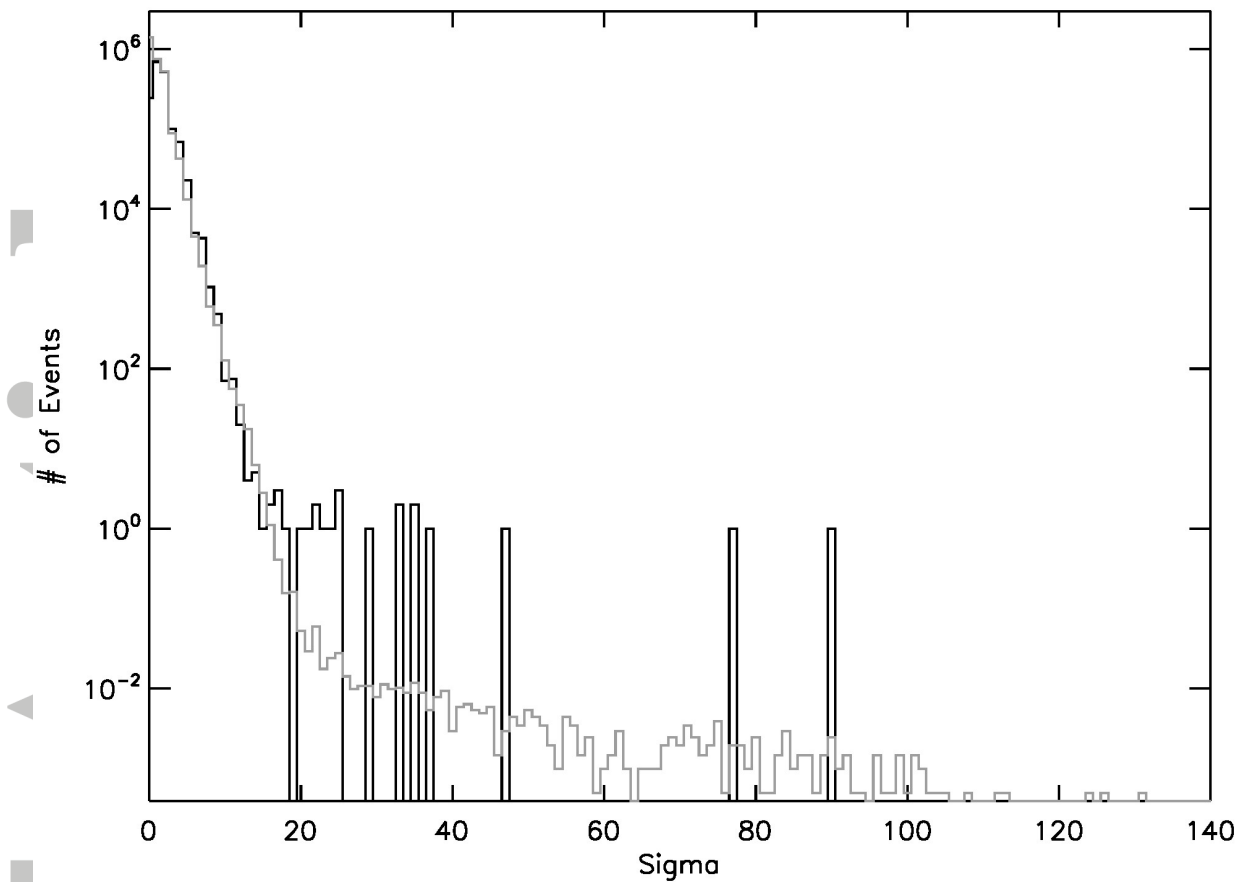
Fig. 4. Distribution of events with significance \sigma . Distribution of events within 7 seconds of nearby ( < 5 miles) lightning is shown in black. Distribution of all data, normalized to 0.52 days of live time, is shown in grey, showing excess of lightning-associated ECs at \sigma > 20 .
