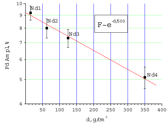
Fig.2: Amplitude of 08/03/12 thermal neutron flux decrease as a function of absorber thickness. Remark: mean absorber thickness for all detectors was obtained as an averaged value after 4\pi integration procedure.
