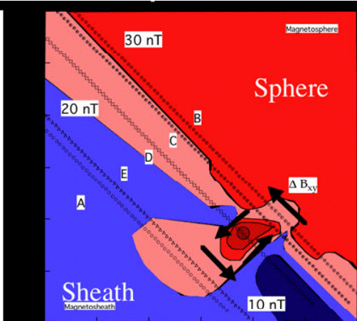
Five THEMIS spacecraft were used to construct cross-sections indicating a flux rope detached from the magnetosphere
