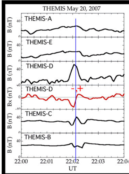
Five THEMIS spacecraft were used to construct cross-sections indicating a flux rope detached from the magnetosphere
