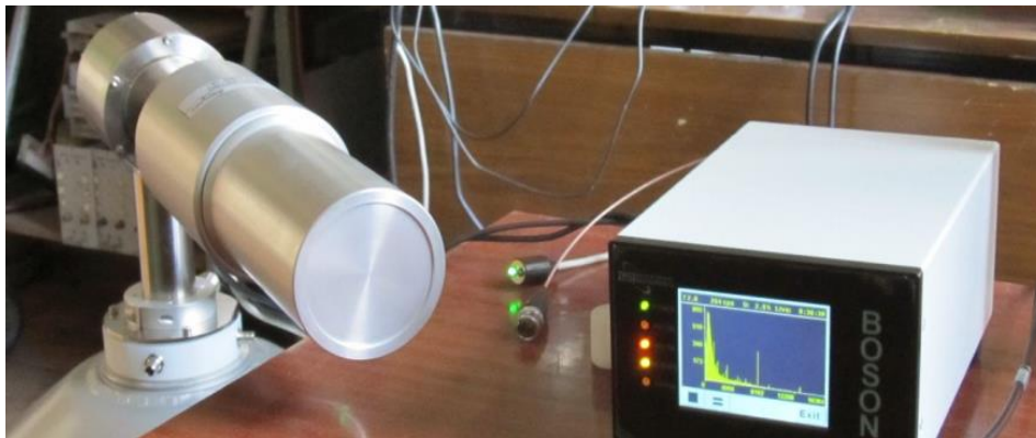
Fig. 3. The new HPGe-detector with its analyzer BOSON
